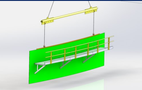
New Shell Plate Installation (Shell + WG + Top Angle)
