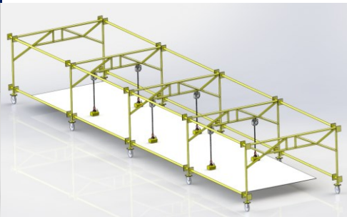
Bottom Plate Moveable Frame
