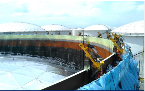
ADR Lifting by Grip Hoist
