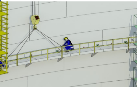
Temporary Wind Girder Working Platform
